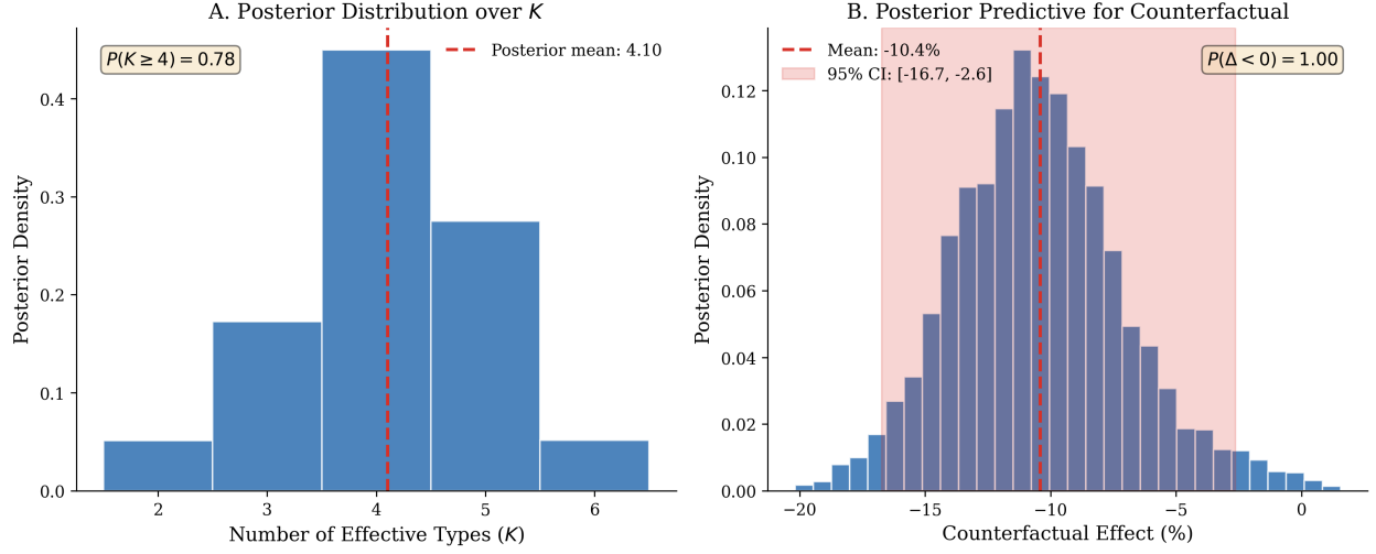
Figure 15: Bayesian Posterior over K and Counterfactual
